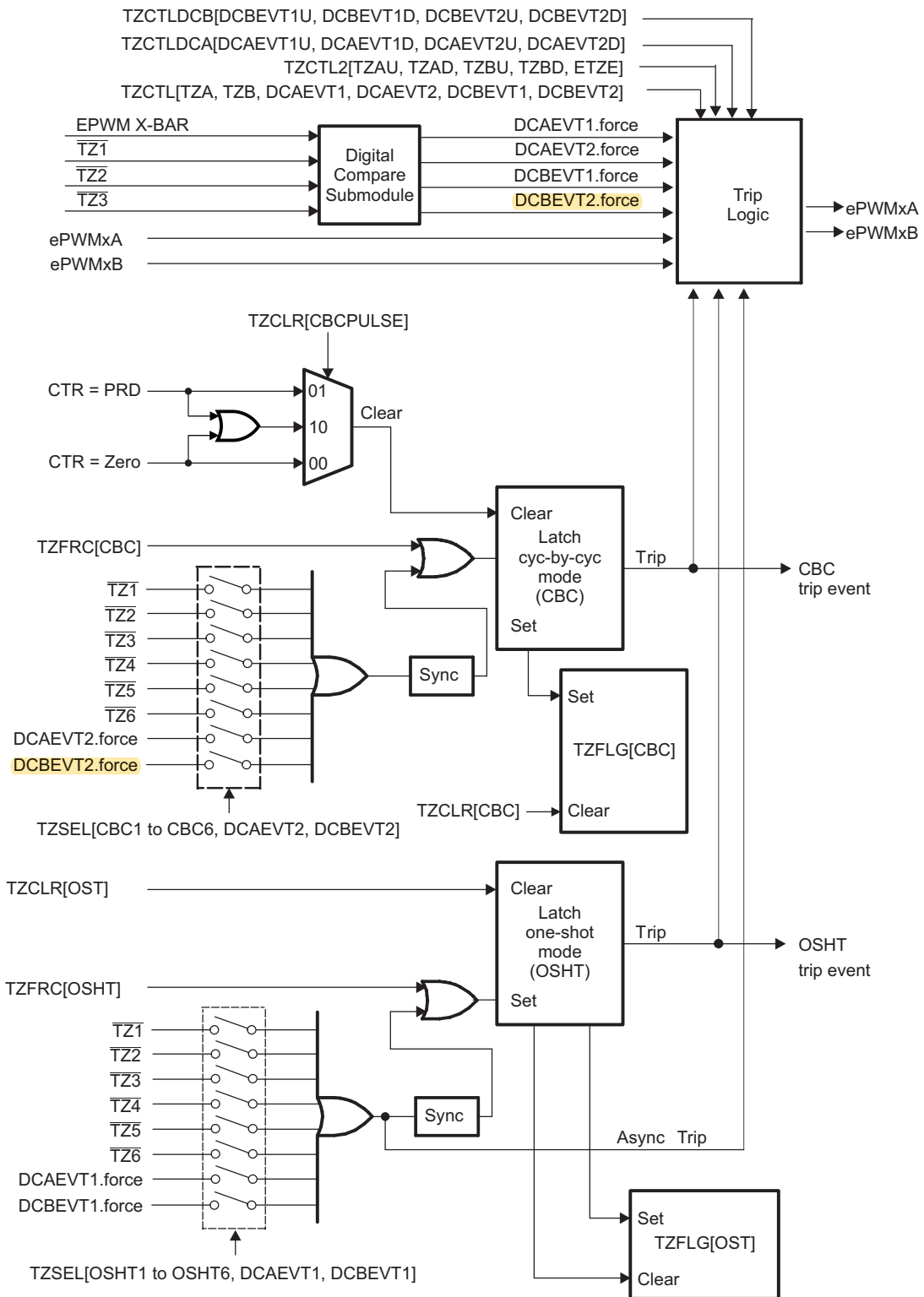
Figure 12-41. Trip-Zone Submodule Mode Control Logic
